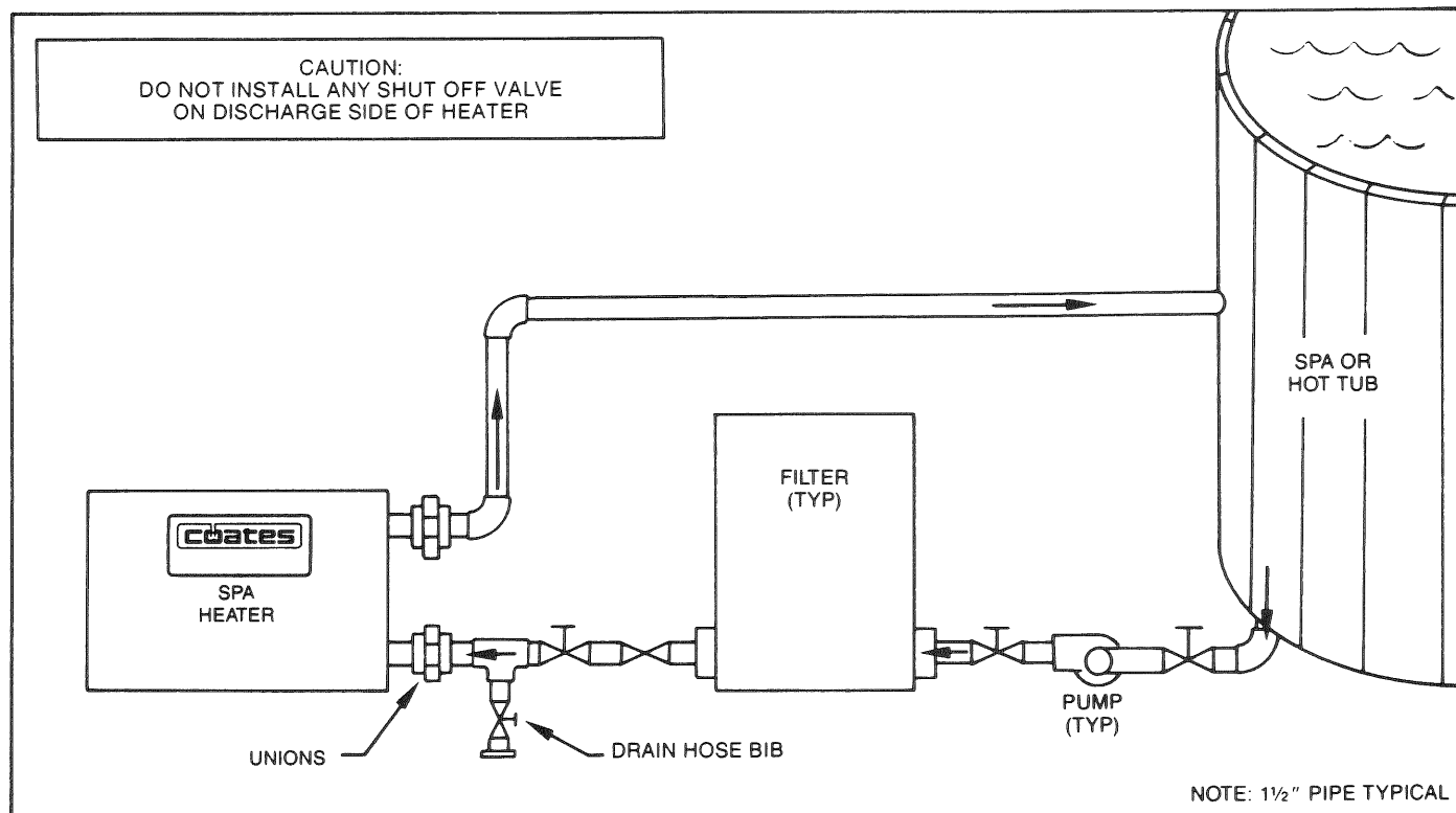
Figure 1. Piping Diagram
