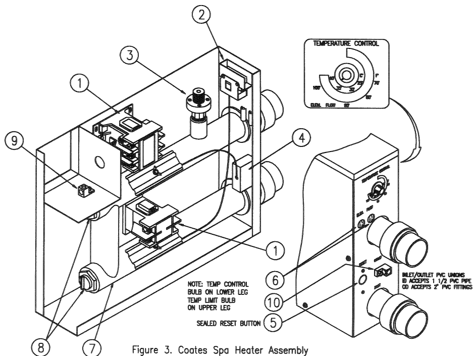
Figure 3. Coates Spa Heater Assembly
